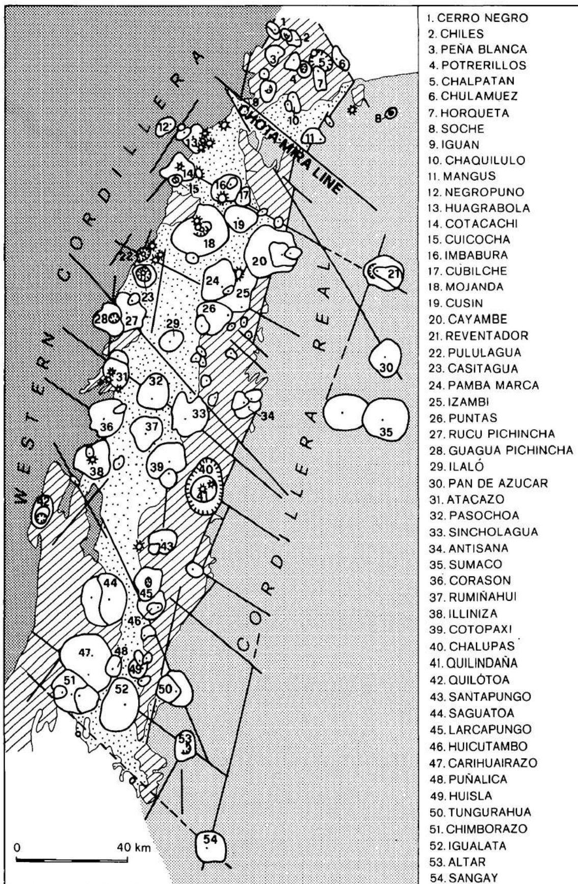
Quaternary volcanoes and main tectonic lineations of the Ecuadorian Andes from 1° N to 2° S.
